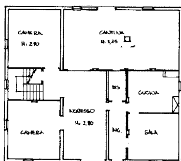
PIANO TERRA
