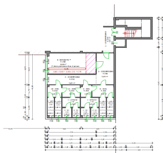
PIANO SEMINTERRATO
