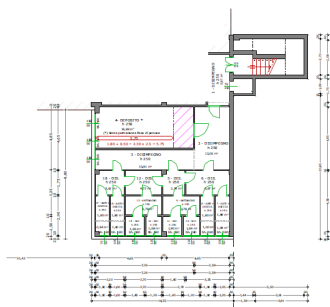
PIANO SEMINTERRATO
